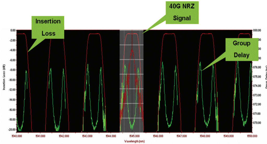
Figure 9. Measurement of insertion loss for an odd/even channel pattern with in-band group delay measurement. Chromatic Dispersion (CD) is derivative of group delay.
