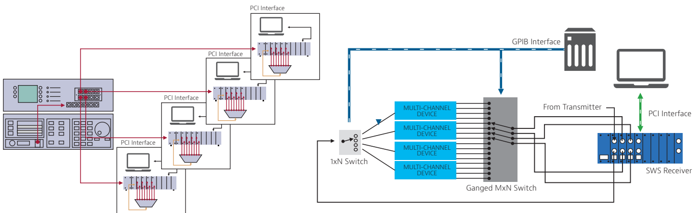
Figure 5. The unique distributed architecture of the VIAVI SWS test system enables the lowest cost of test while still maintaining the speed of measurement and scanning range required for ROADM components. Optical switches can improve capital utilization and increase the number of modules that can be tested at an individual station.
