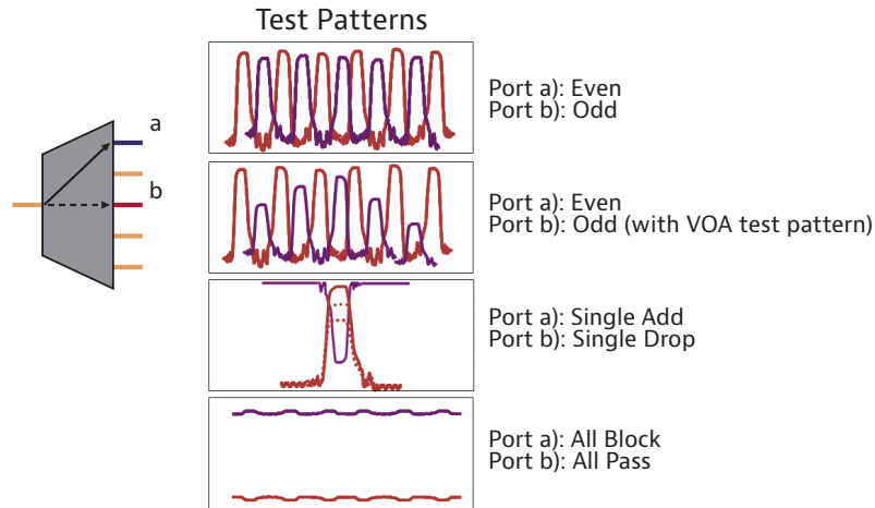
Figure 4. Example test patterns for a WSS showing some of the more challenging test states. These patterns can be replicated across many different channel pairs.
