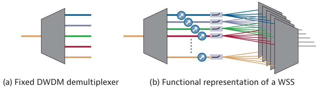
Figure 2. Functional difference between fixed DWDM demultiplexer and a WSS. The fixed demultiplexer (a) separates specific wavelengths to a fixed output fiber. The WSS (b) allows any wavelength to be mapped to any output fiber and is functionally equivalent to over 150 discrete components.
