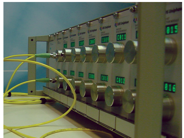
Figure 1. VIAVI SWS Test Station for DWDM Component and Module Measurements
